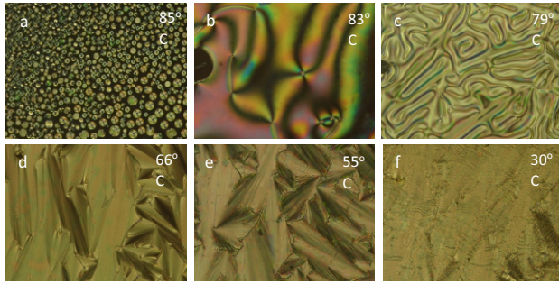
Figure 3. Micrographs of FLC in 10 μm cell with anti parallel rubbing at different temperature showing (a) Formation of nucleation (b) nematic phase (c) cholesteric phase (d) Sm A phase (e) focal conic texture (f) SmC* phase.
