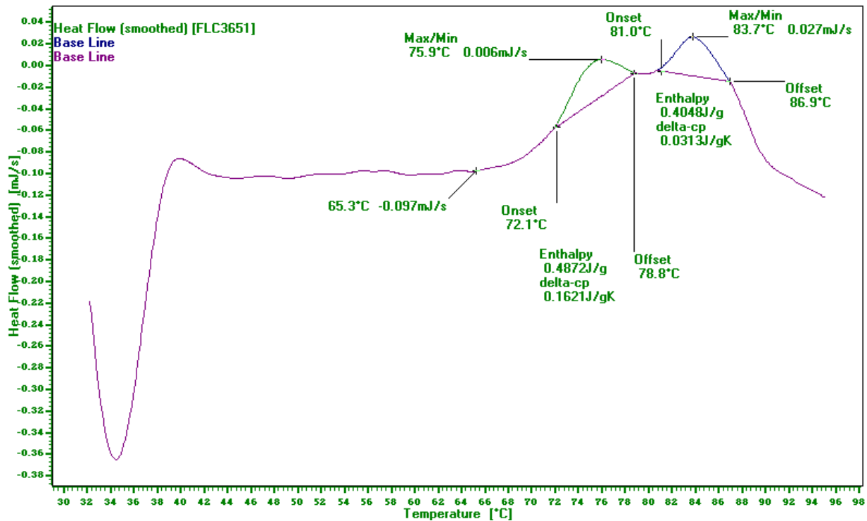
Figure 4. shows the DSC graph for ZLI 3651 FLC material. The phase sequence of the material can be obtained by identifying various phases of LCs as shown below:
