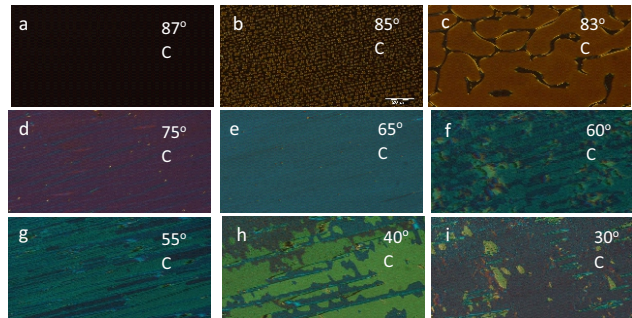
Figure 2. (a) Microscopic textures of ZLI 3651 obtained during cooling below isotropic temperature in 5\mu\text{m} thickness cell shows (a) Isotropic phase (b) & (c) nucleation growth (d) Cholesteric phase (e) hair pin defects (f) SmA phase (g) SmC* phase (h) formation of domains and (i) microscopic texture at room temperature.
