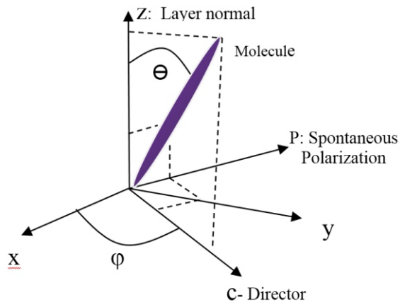
Figure 1. Projection of molecule in SmC* phase
