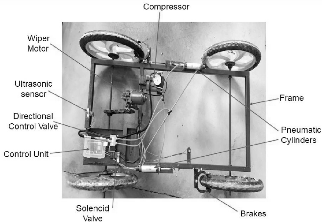
Figure3. Experimental setup
