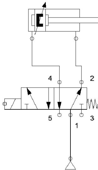
Figure 5. Pneumatic braking circuit
