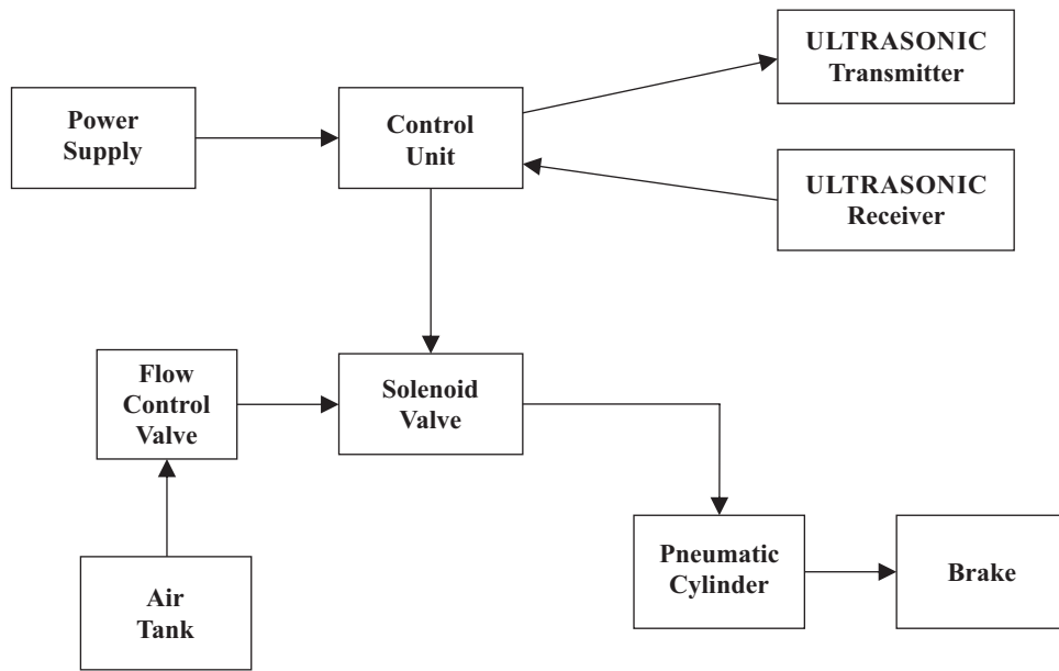
Figure 4. Block diagram of experimental setup
